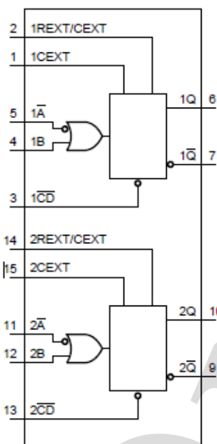
Figure 1. Functional diagram
