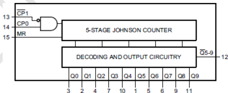
Figure 3. Functional diagram
