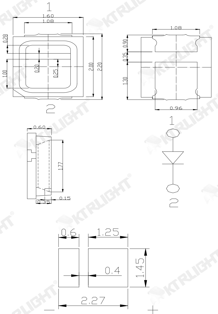
推荐焊盘式样 (Recommended Soldering Patter)
