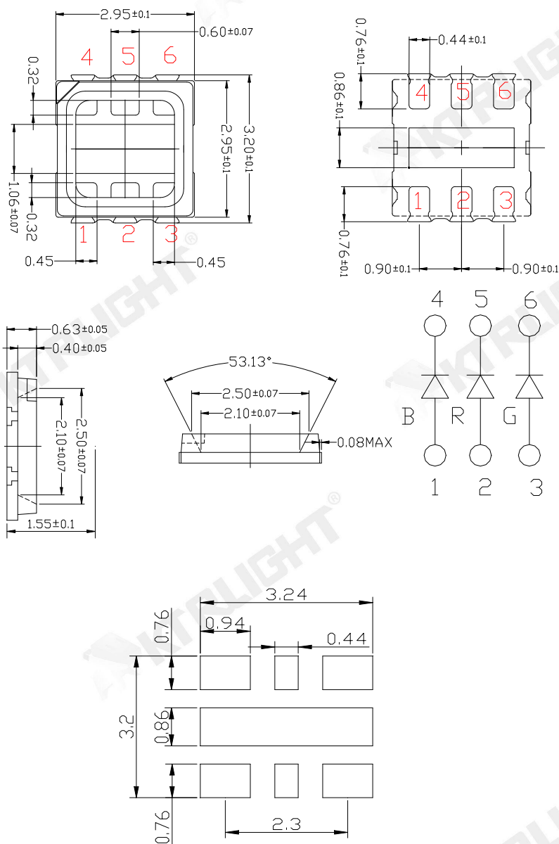
推荐焊盘式样 (Recommended Soldering Patter)
