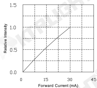
Relative Intensity vs. Forward Current (Ta=25°C)
