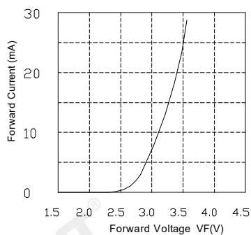
Forward Voltage vs. Forward Current (Ta=25°C)
