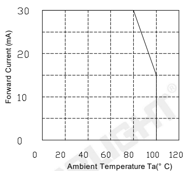
Ambient Temperature vs. Maximum Forward Current
