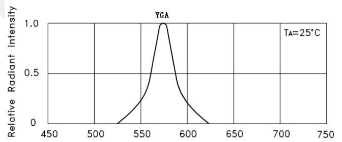
wavelength \lambda (nm) RELATIVE INTENSITY Vs. WAVELENGTH
