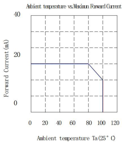
Detrating
