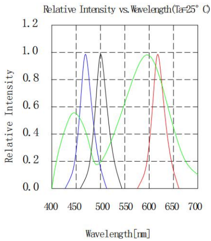
Spectral Distribution
