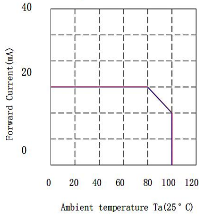
Ambient temperature vs. Maximum Forward Current
