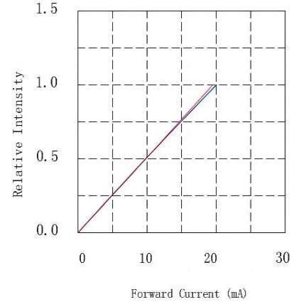
Relative Intensity vs. Forward Current (Ta=25°C)
