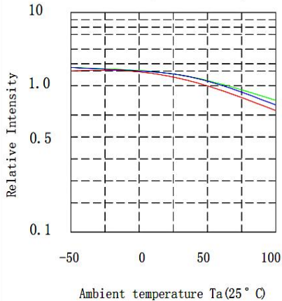
Relative Intensity vs. Ambient temperature
