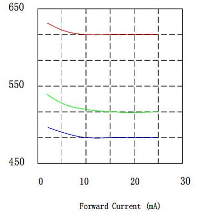
Forward Current vs. Chromaticity (Ta=25°C)
