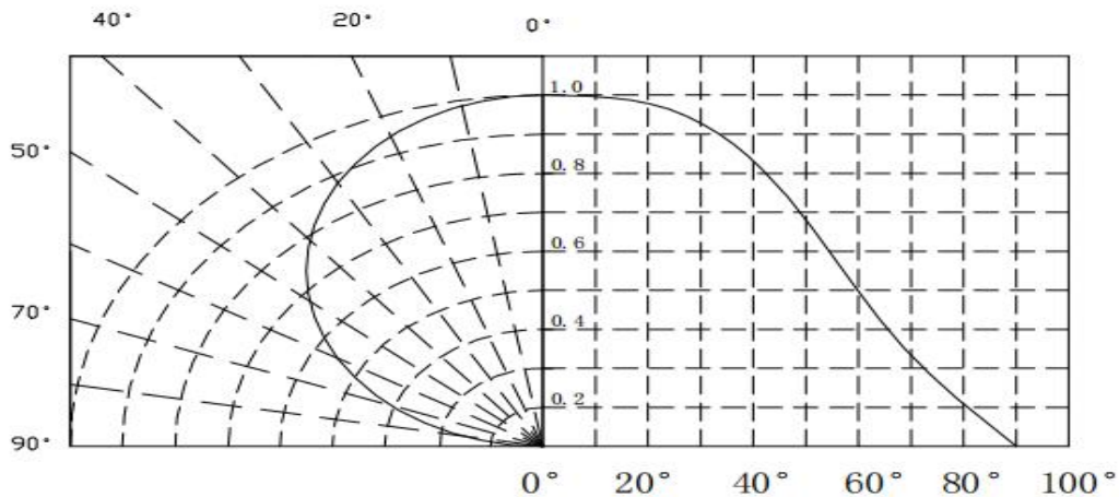
Diagram characteristics of radiation
