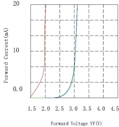
Forward current vs. Forward Voltage (Ta=25°C)
