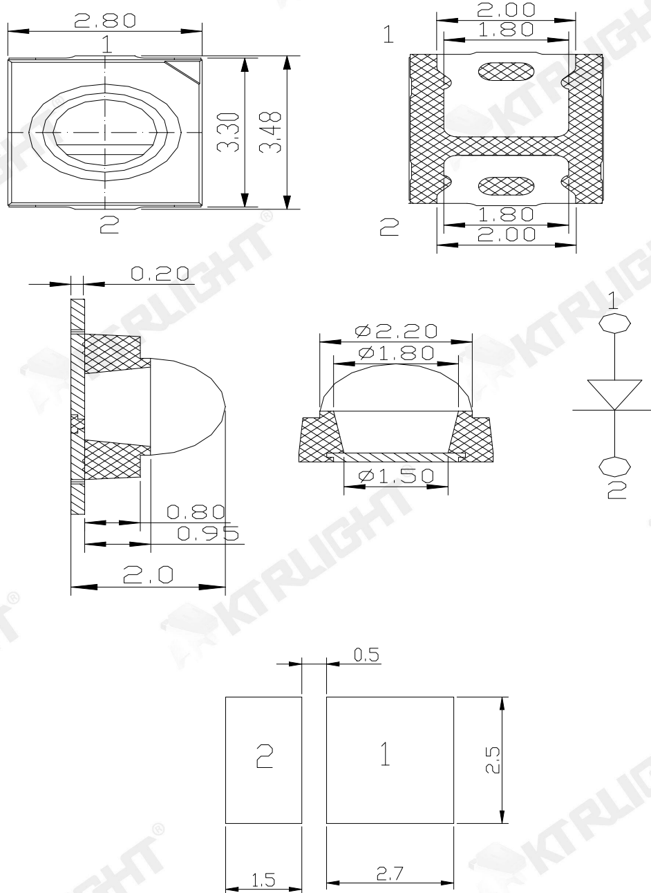
推荐焊盘式样(Recommended Soldering Patter)
