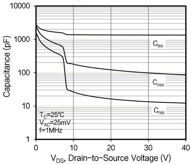
Figure 7. Capacitance
