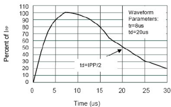
Pulse Waveform
