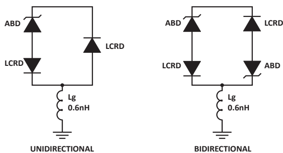
FIGURE 1 SPICE MODEL
