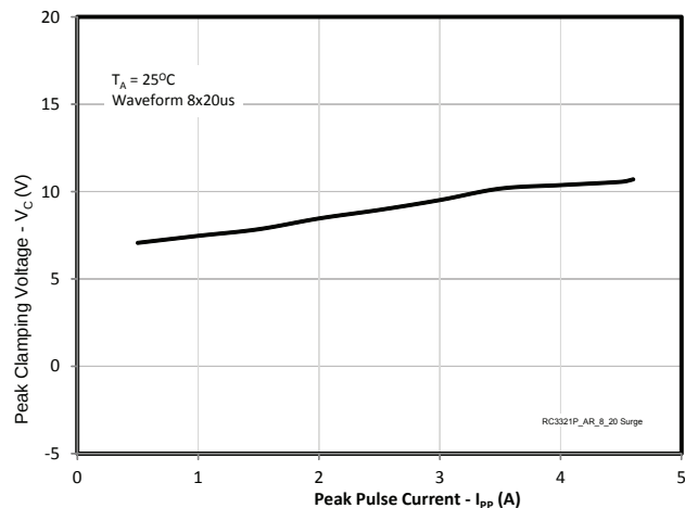
8x20us Peak Clamping Voltage vs Peak Current
