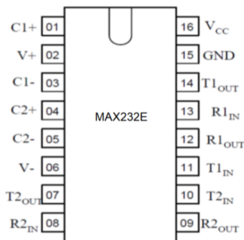
Pin configuration
