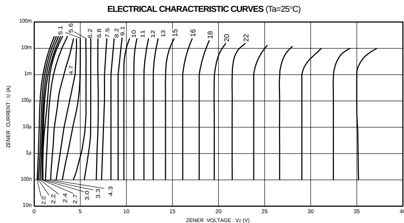
Fig.1 Zener voltage characteristics
