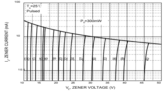
Zener Characteristics (11 V to 43 V)
