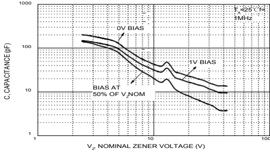
Typical Capacitance
