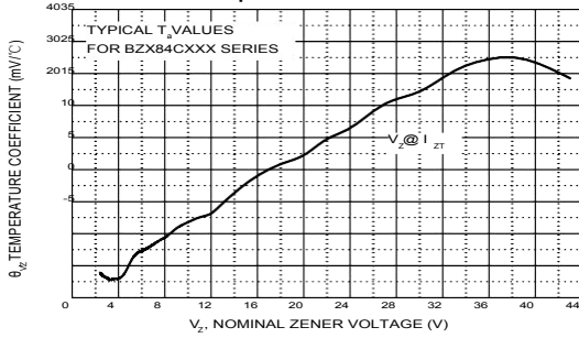
Temperature Coefficients
