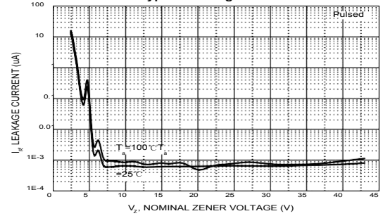
Typical Leakage Current
