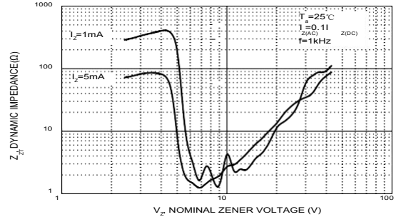
Effect of Zener Voltage on Zener Impedance
