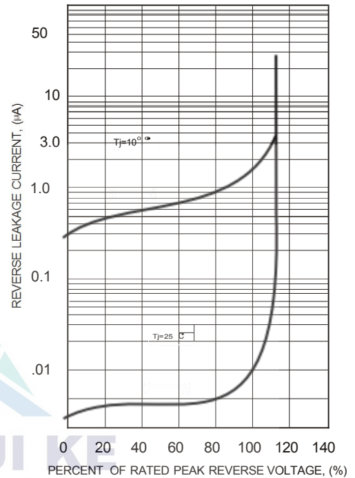
FIG.4-TYPICAL REVERSE CHARACTERISTICS
