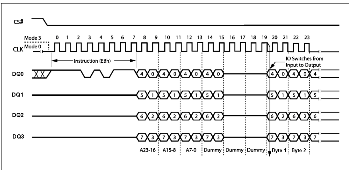
Figure 18. Quad Input / Output Fast Read Instruction Sequence Diagram
