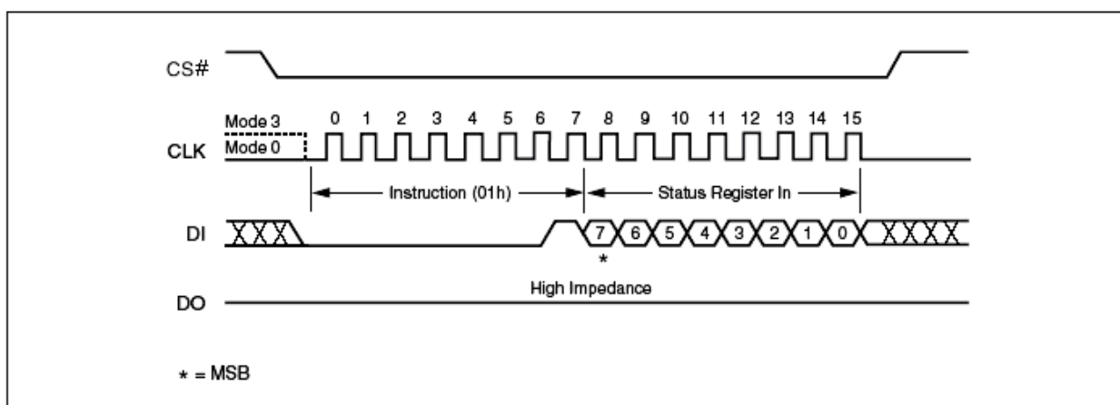
Figure 13. Write Status Register Instruction Sequence Diagram
