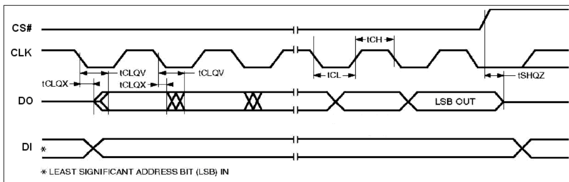
Figure 39. Serial Output Timing
