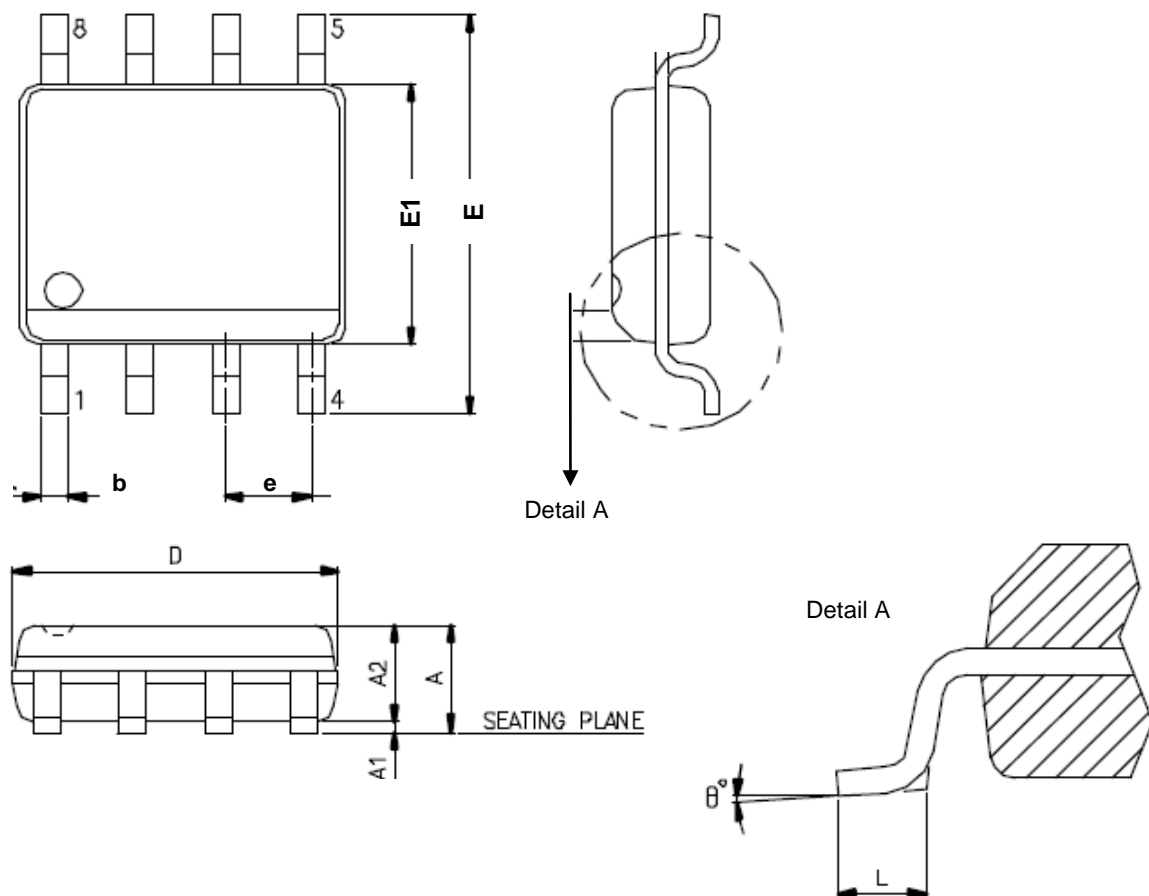
Figure 47. SOP 8 (150 mil)
