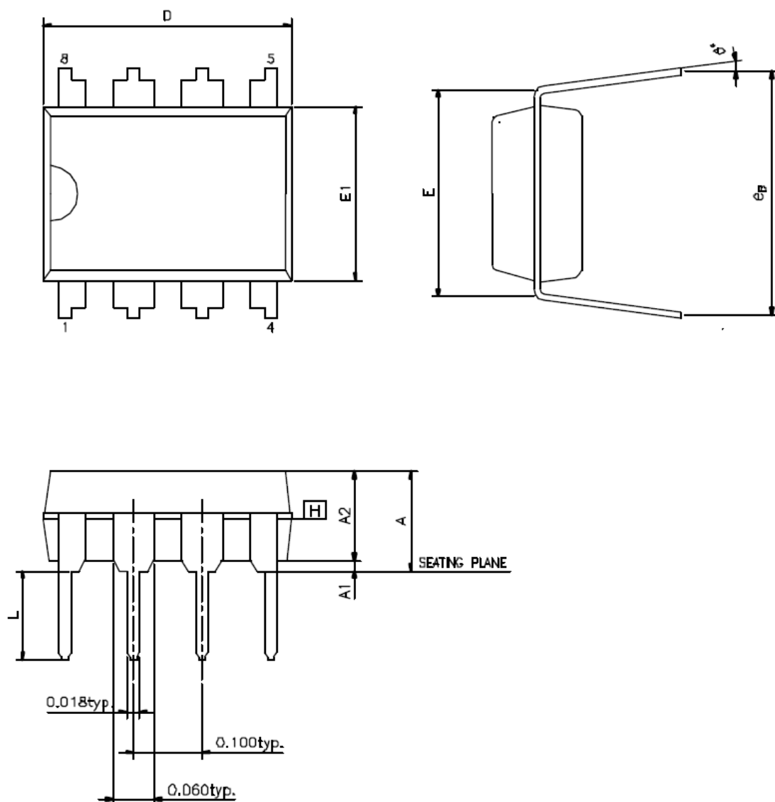
Figure 53. PDIP8
