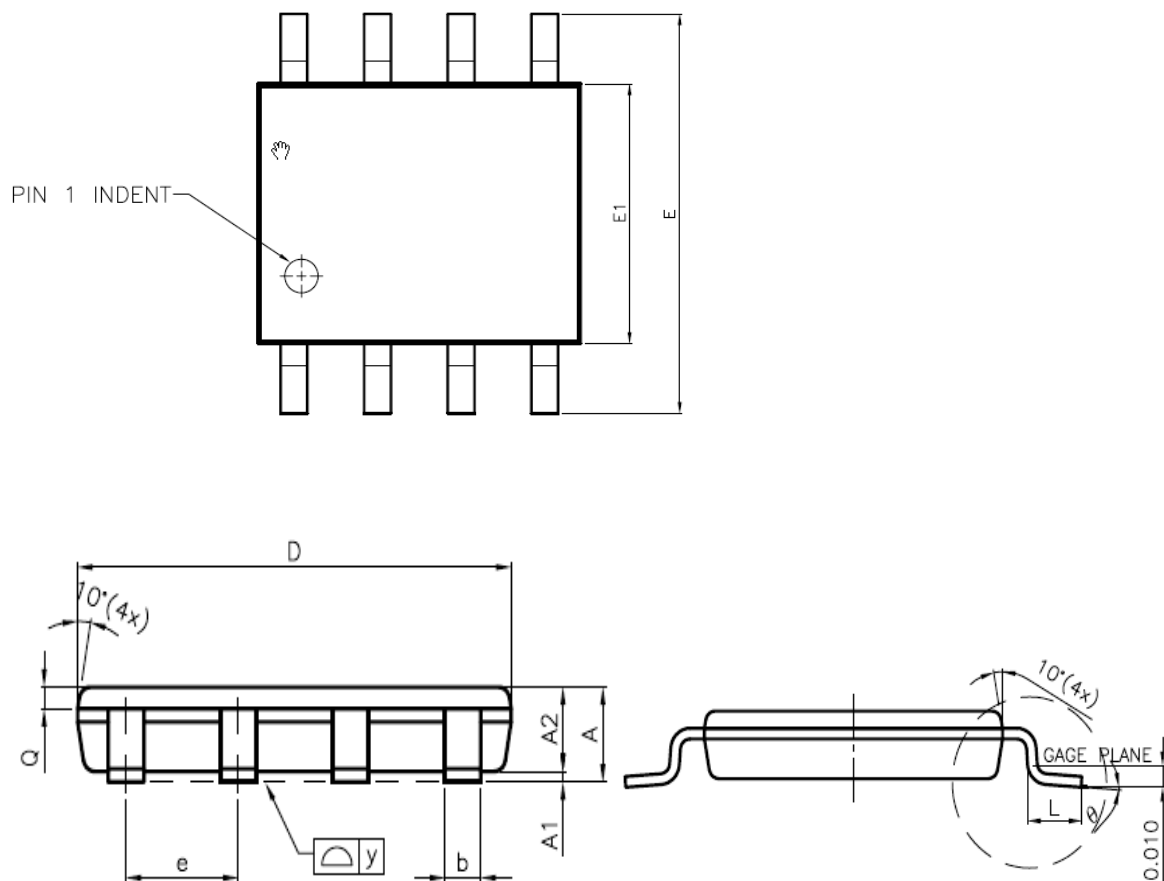
Figure 48. VSOP 8 (150mil)
