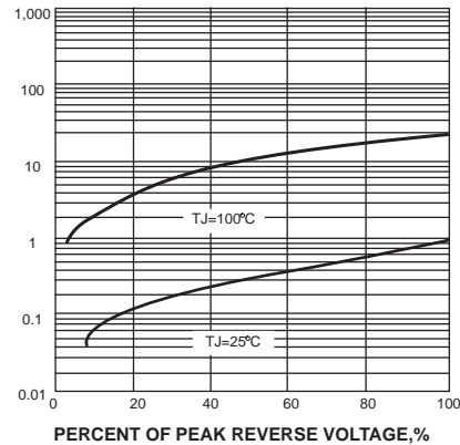
FIG. 4-TYPICAL REVERSE CHARACTERISTICS
