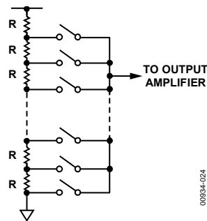
Figure 24. Resistor String
