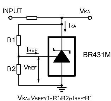
Test Circuit for V_{KA} \geq V_{REF}
