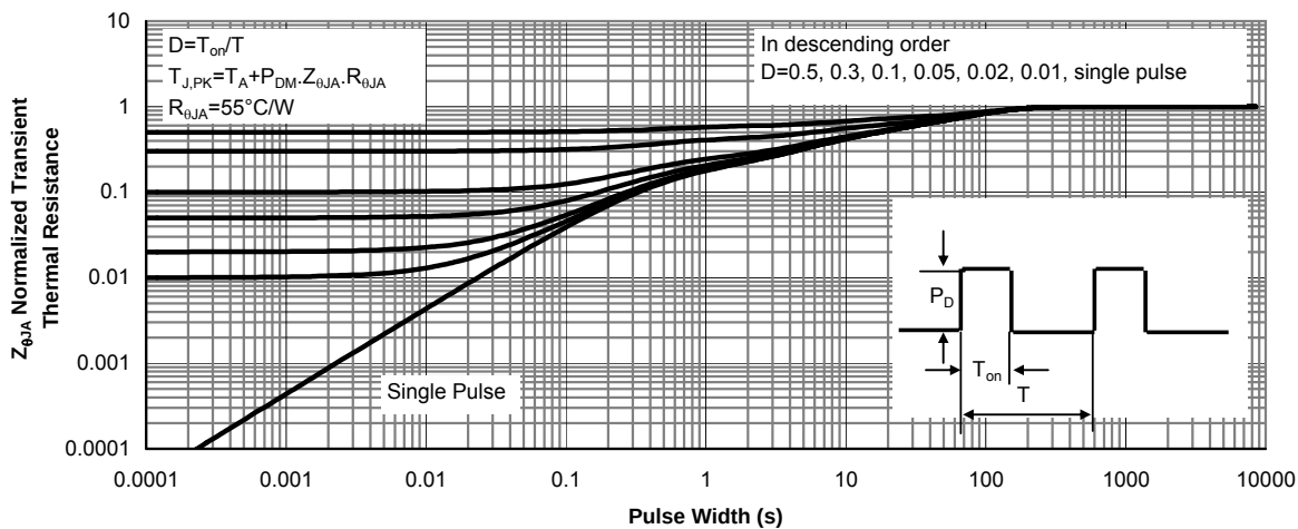
Figure 15: Normalized Maximum Transient Thermal Impedance (Note G)
