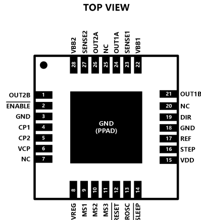
QFN28
