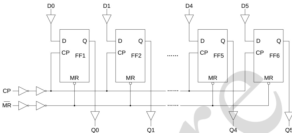
Figure 1. Logic diagram
