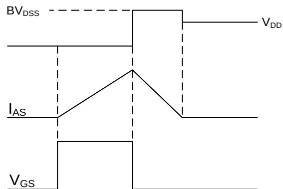
Fig.8 EAS Waveform
