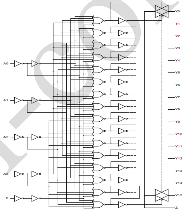
Figure 2. Logic diagram
