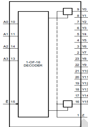
Figure 1. Functional diagram
