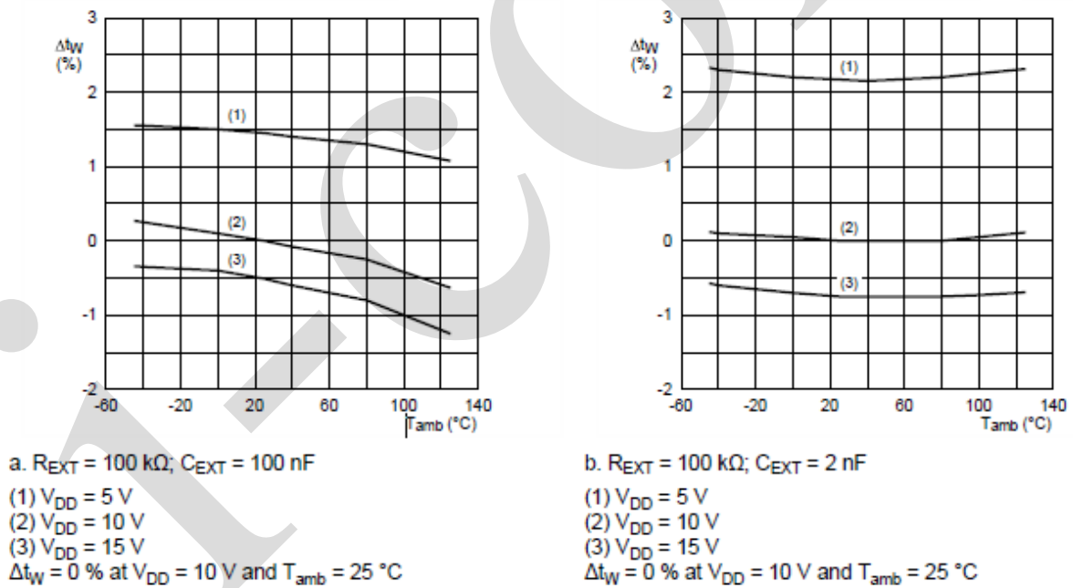
Figure 6. Typical normalized change in output pulse width as a function of ambient temperature
