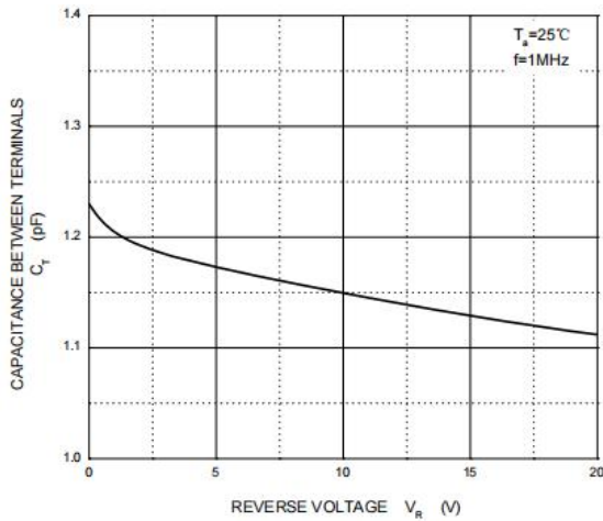
Figure 3: Capacitance Characteristics
