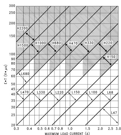
XL2576-ADJ
