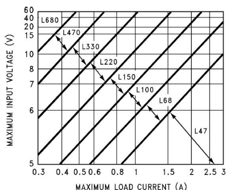
XL2576-3.3
