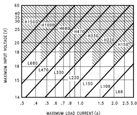
XL2576-12
