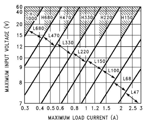
XL2576-5.0
