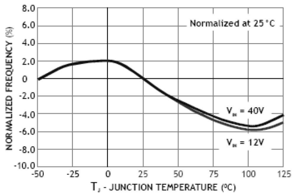
OSCILLATOR FREQUENCY
