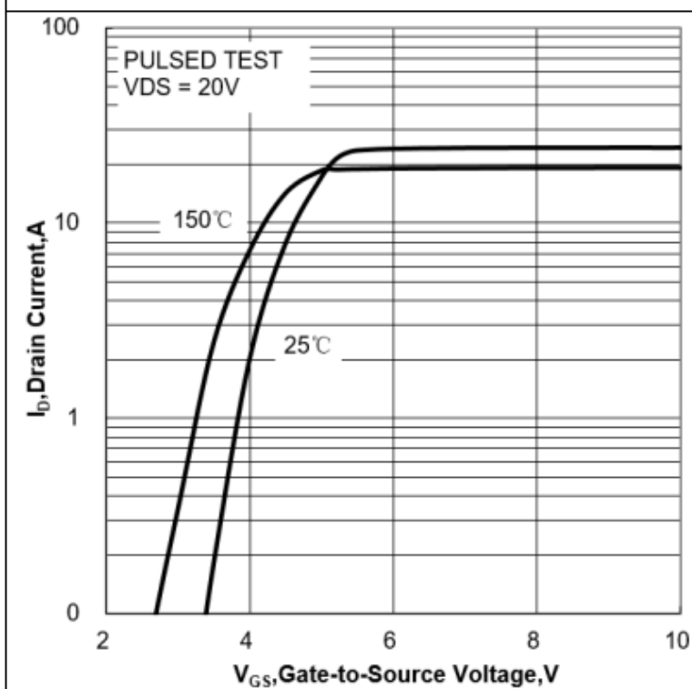
Figure 5 Typical Transfer Characteristics
