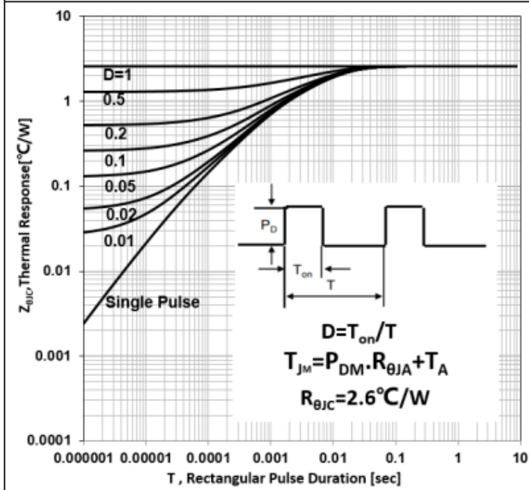
Figure 3c Max Thermal Impedance (TO-220F)
