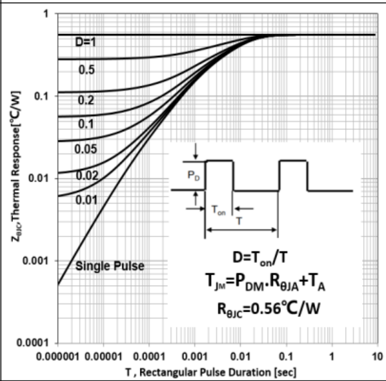
Figure 3b Max Thermal Impedance (TO-220)
