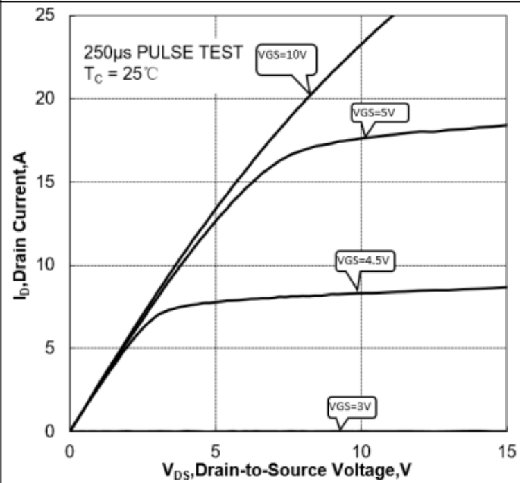
Figure 4 Typical Output Characteristics
