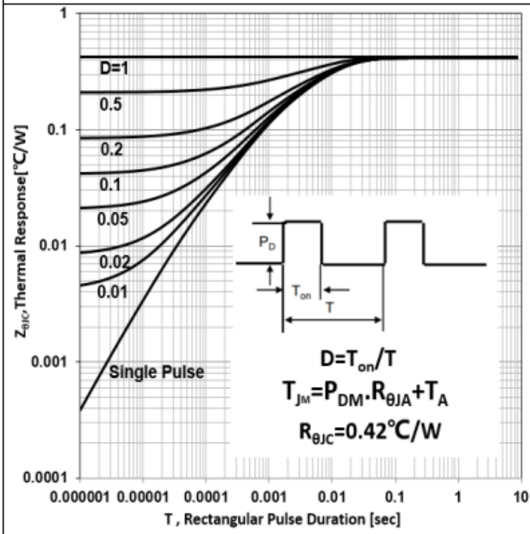
Figure 3a Max Thermal Impedance (TO-3PN)
