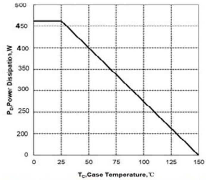
Figure 2 Maximum Power dissipation vs Case Temperature
