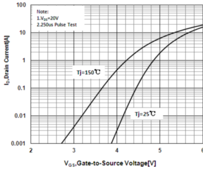
Figure 6 Typical Transfer Characteristics
