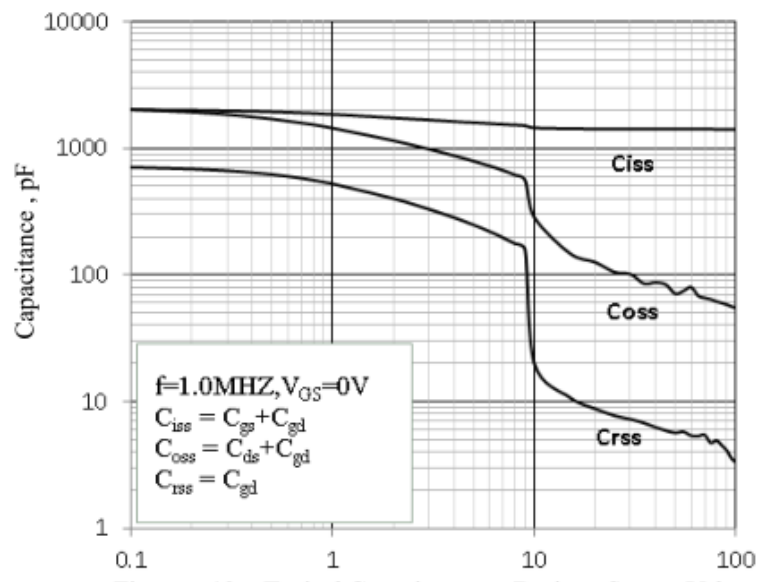
Figure 13 Typical Capacitance vs Drain to Source Voltage
