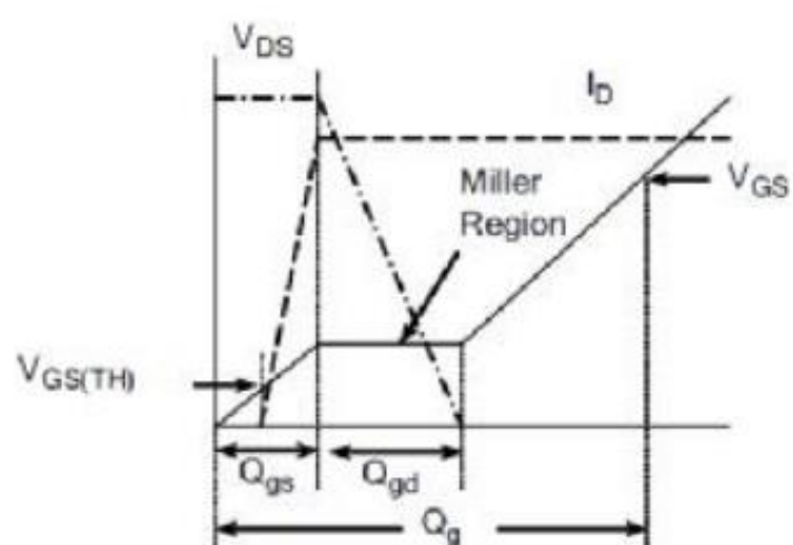
Figure 18. Gate Charge Waveform
