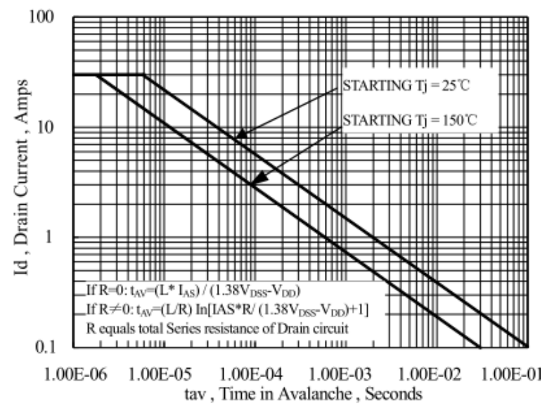
Figure 16 Unclamped Inductive Switching Capability
