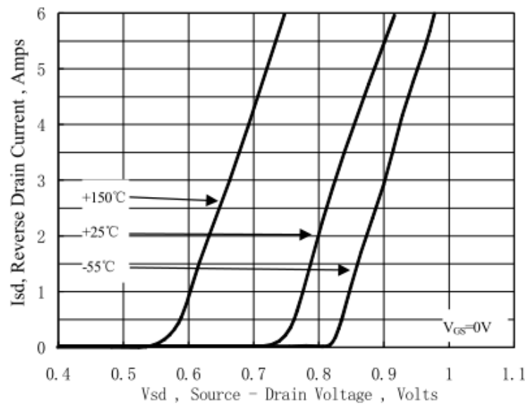
Figure 15 Typical Body Diode Transfer Characteristics
