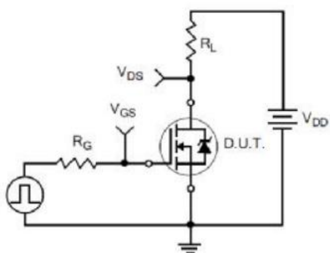
Figure 19. Resistive Switching Test Circuit
