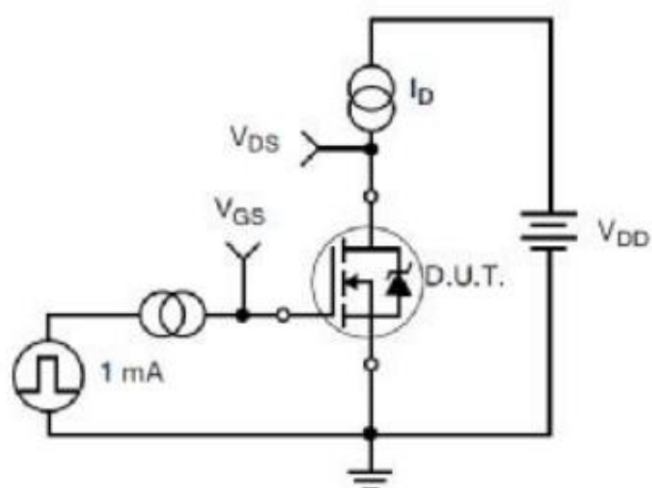
Figure 17. Gate Charge Test Circuit
