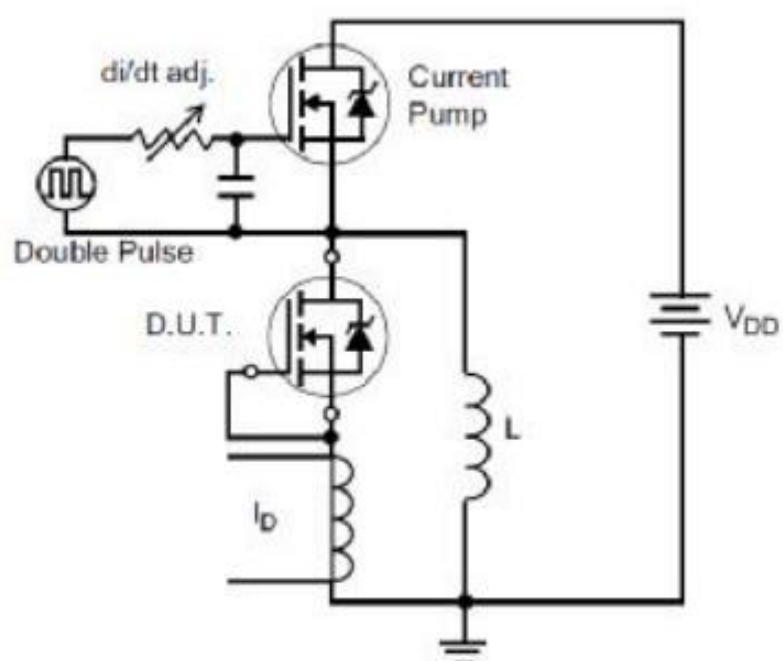
Figure 21. Diode Reverse Recovery Test Circuit
