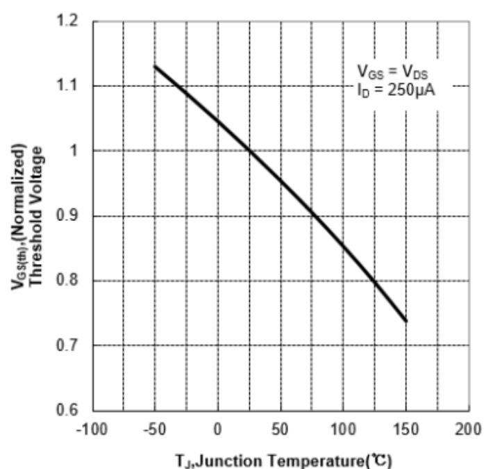
Figure 8 Typical Threshold Voltage vs Junction Temperature
