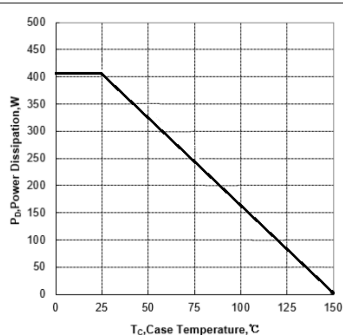
Figure 2 Power Dissipation
