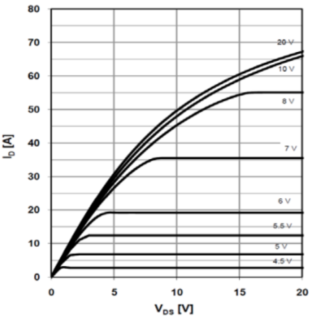
Typ. output characteristics T_J=25\text{ }^{\circ}\text{C} parameter: V_{GS}
