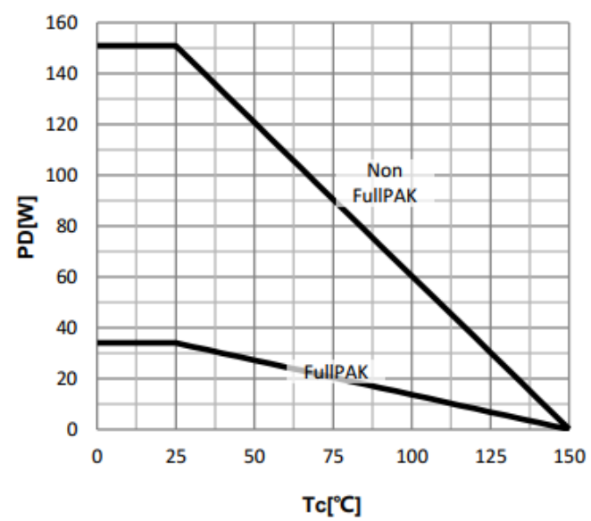
Power dissipation
