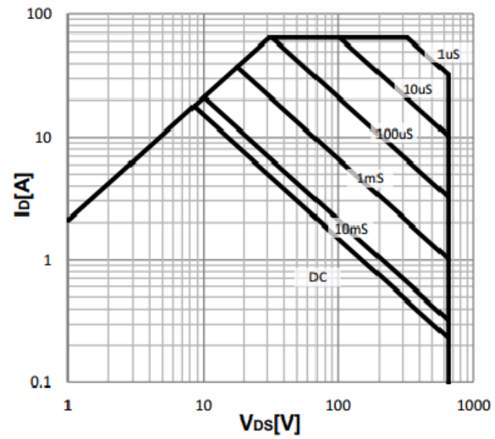
Safe operating area T_C=25^{\circ}\text{C}
