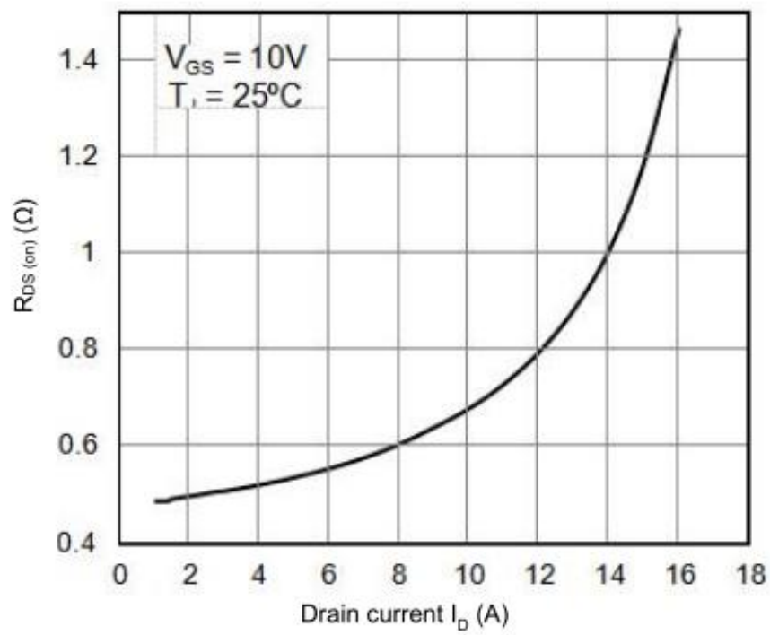
Figure 3. On-Resistance vs. Drain Current
