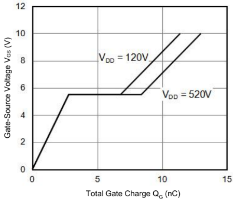
Figure 5. Gate Charge Characteristics
