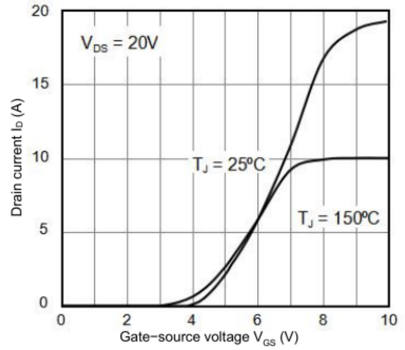
Figure 2. Transfer Characteristics
