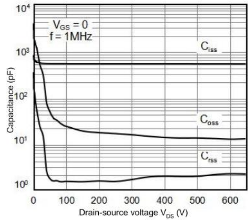
Figure 4. Capacitance Characteristics
