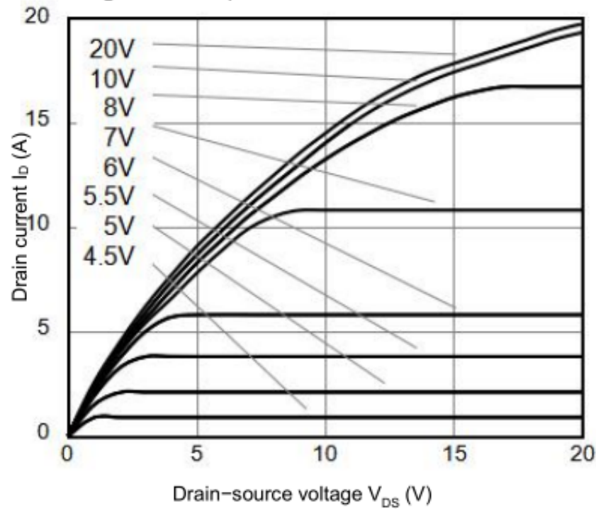
Figure 1. Output Characteristics
