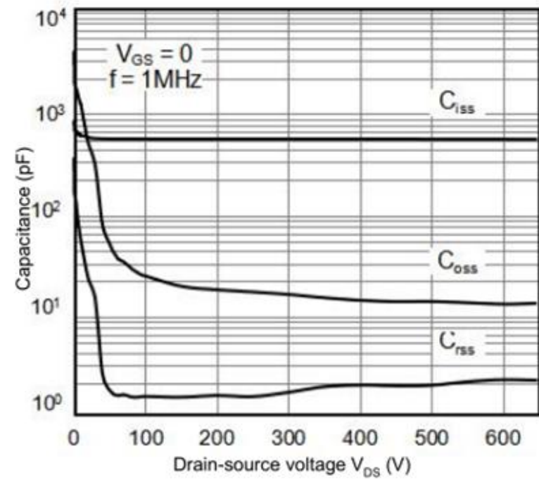
Figure 4. Capacitance Characteristics
