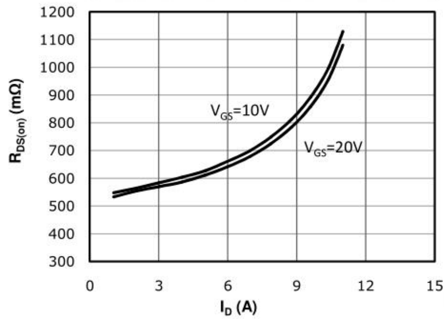
Figure 3. On-Resistance vs. Drain Current
