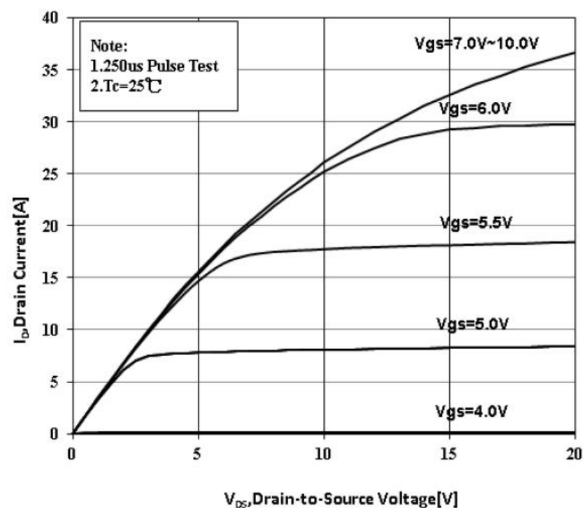
Figure 4 Typical Output Characteristics
