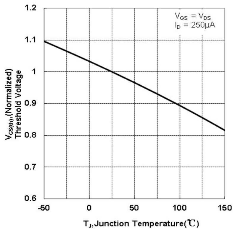
Figure 10 Typical Theshold Voltage vs Junction Temperature
