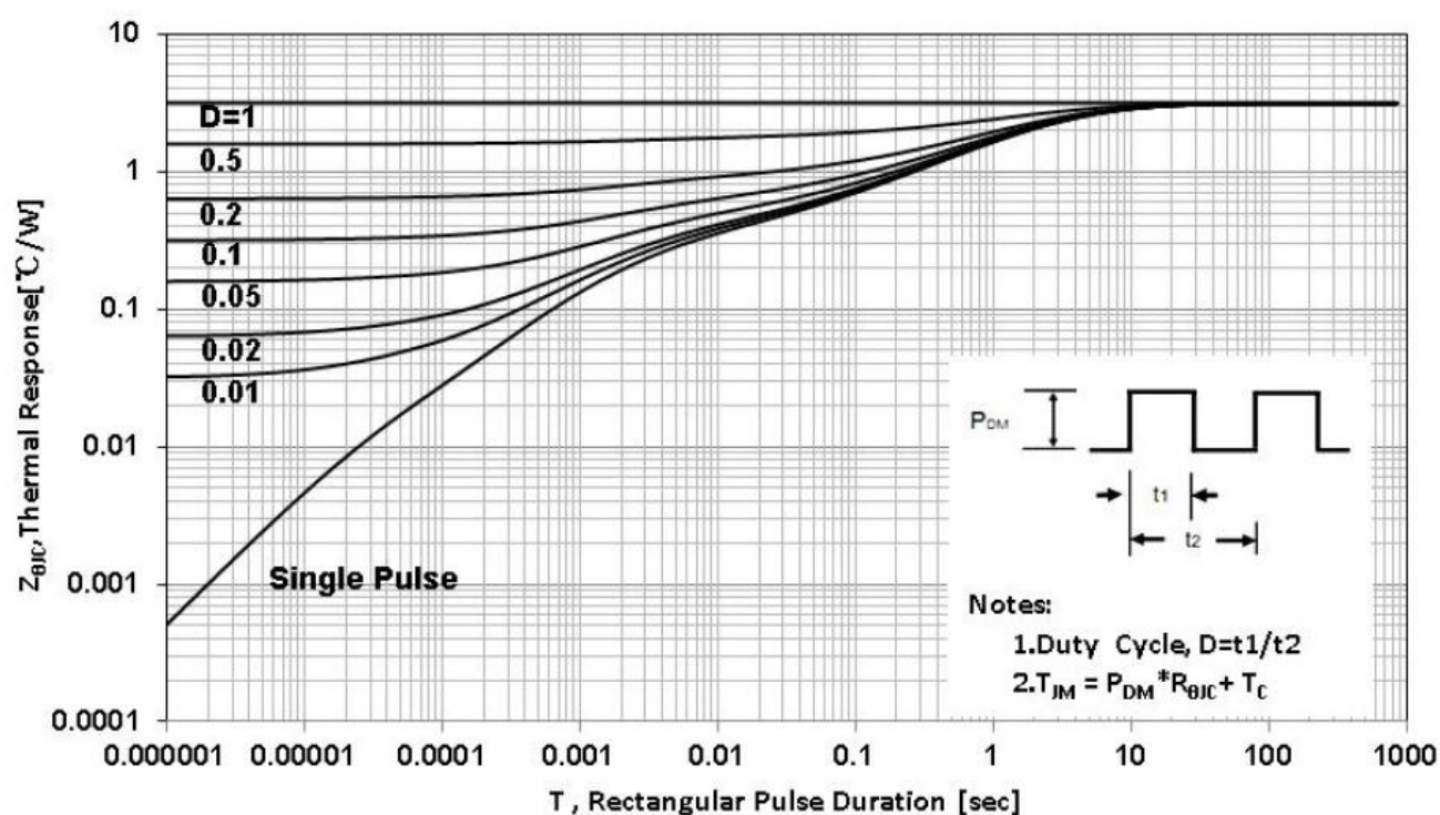
Figure 5 Maximum Effective Thermal Impedance, Junction to Case
