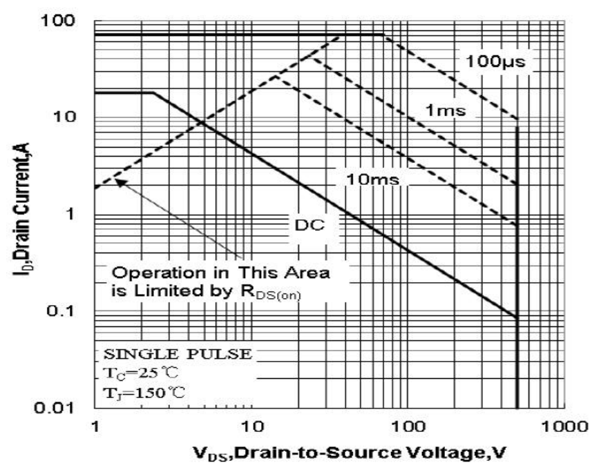
Figure 1 Maximum Forward Bias Safe Operating Area
