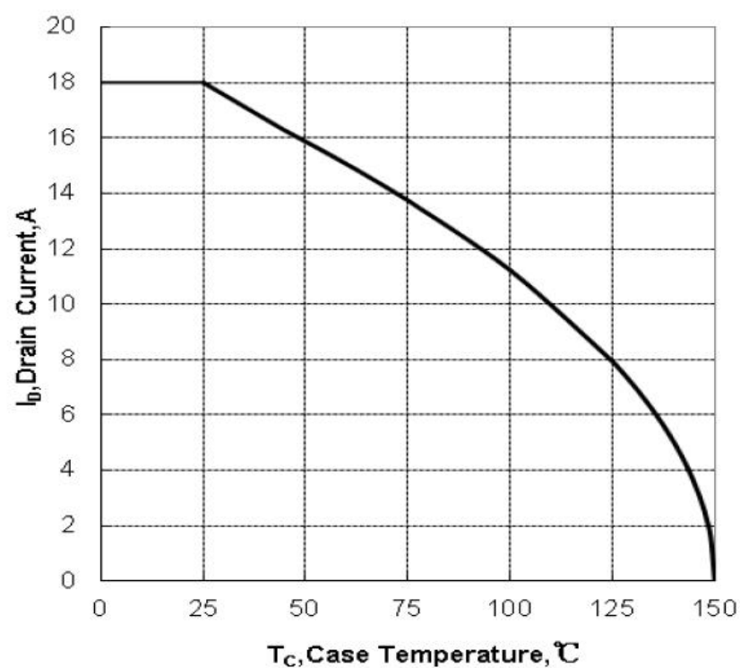
Figure 3 Maximum Continuous Drain Current vs Case Temperature
