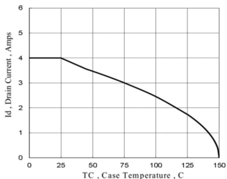
Figure 3 Maximum Continuous Drain Current vs Case Temperature
