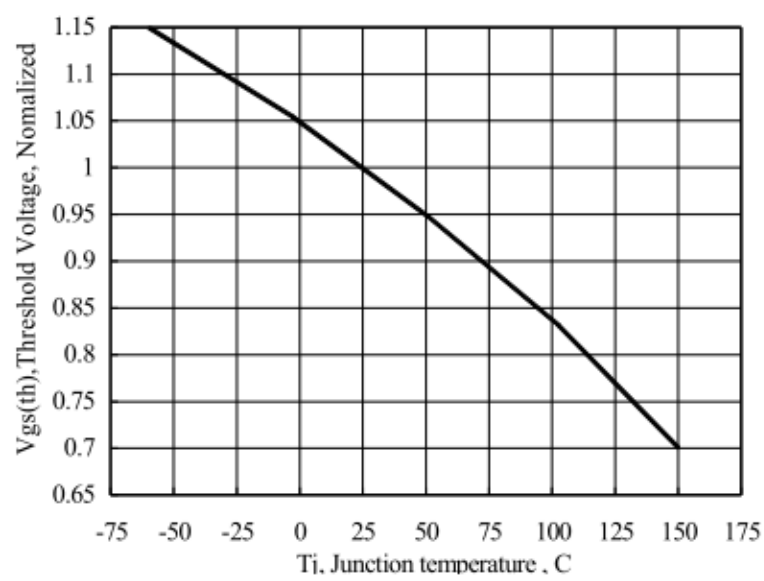
Figure 10 Typical Theshold Voltage vs Junction Temperature
