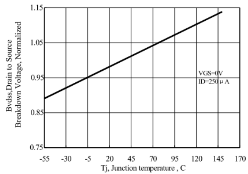
Figure 11 Typical Breakdown Voltage vs Junction Temperature
