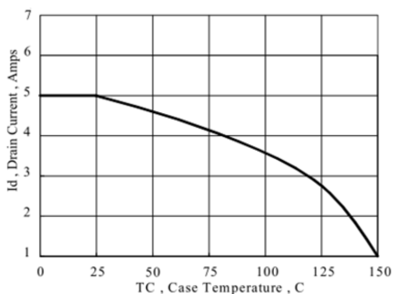
Figure 3 Maximum Continuous Drain Current vs Case Temperature
