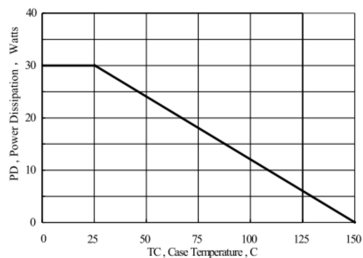
Figure 2 Maximum Power Dissipation vs Case Temperature
