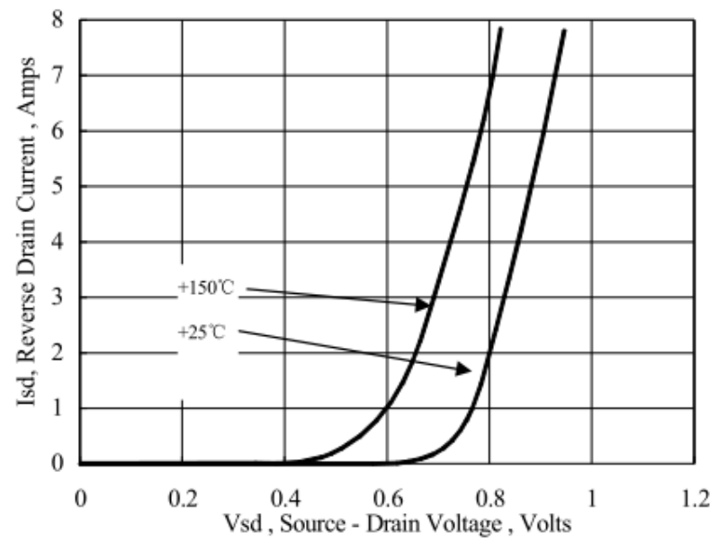
Figure 7 Typical Body Diode Transfer Characteristics
