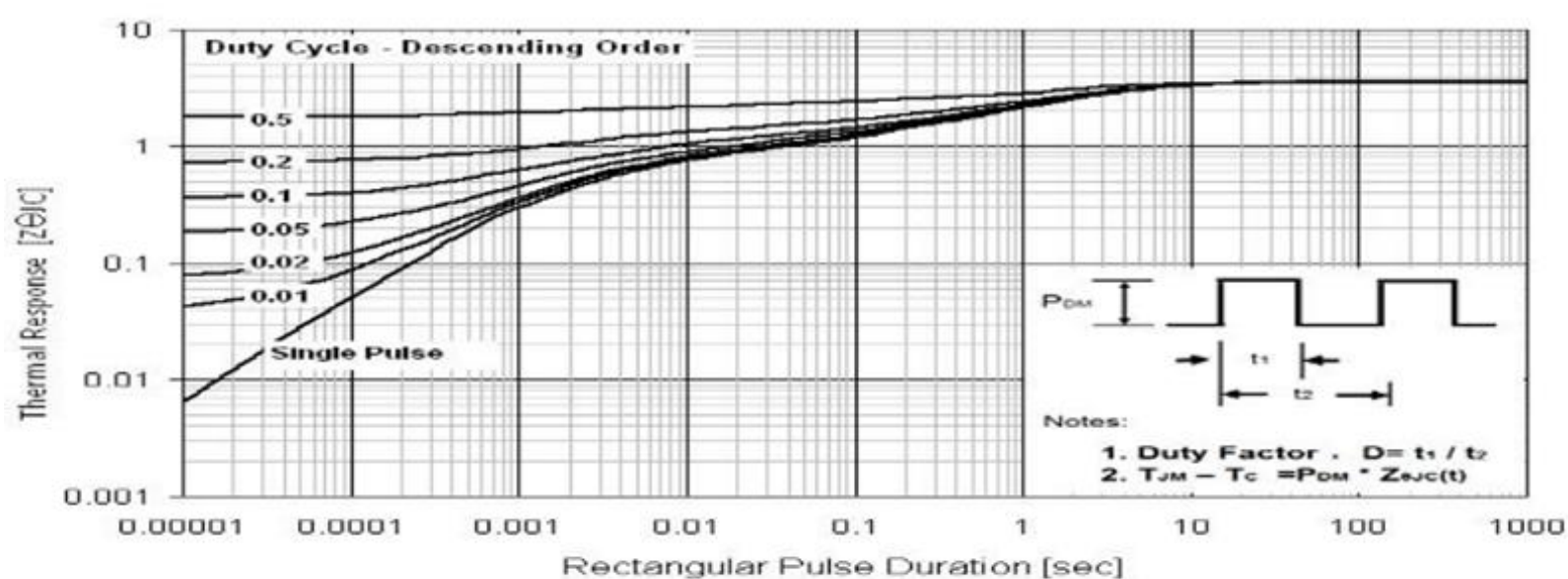
Figure 5 Maximum Effective Thermal Impedance, Junction to Case
