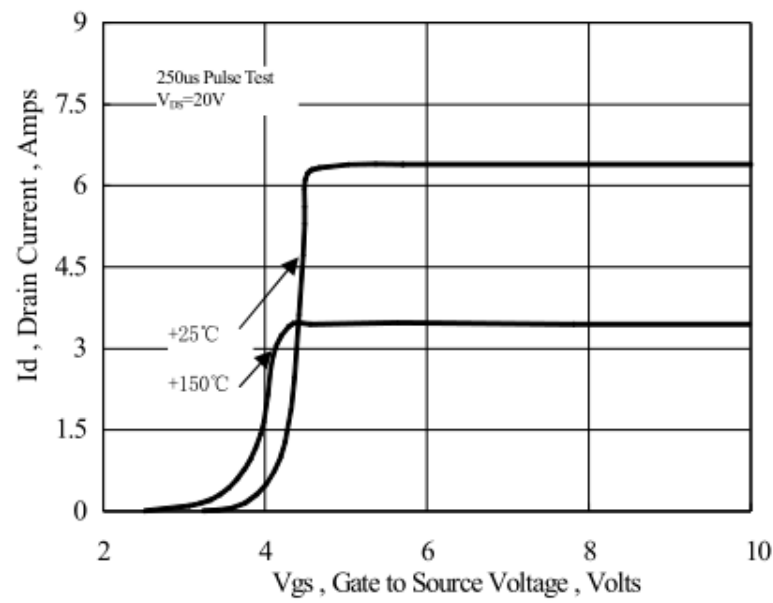
Figure 6 Typical Transfer Characteristics
