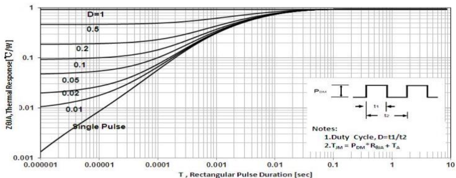
Figure 5 Maximum Effective Thermal Impedance. Junction to Case
