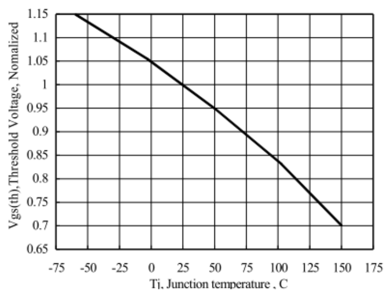
Figure 10 Typical Threshold Voltage vs Junction Temperature
