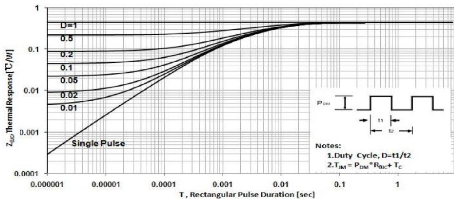
Figure 5 Maximum Effective Thermal Impedance, Junction to Case
