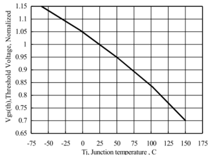
Figure 10 Typical Threshold Voltage vs Junction Temperature
