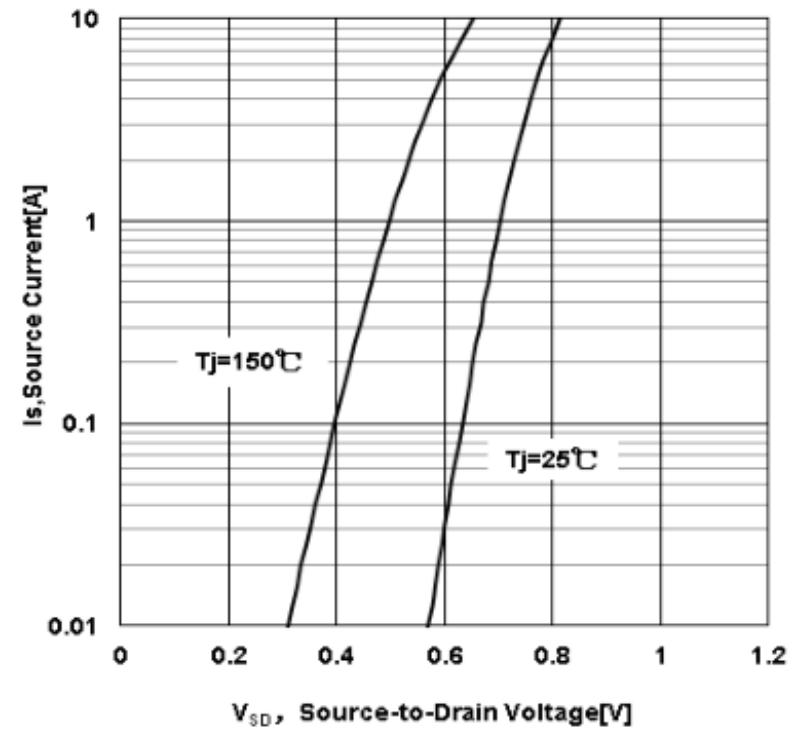
Figure 7 Typical Body Diode Transfer Characteristics
