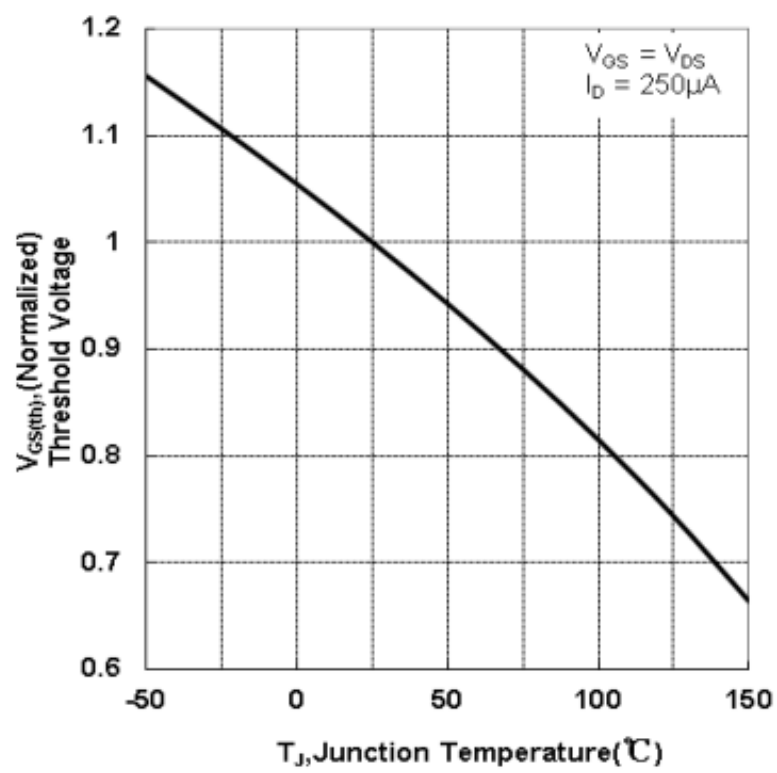
Figure 10 Typical Threshold Voltage vs Junction Temperature
