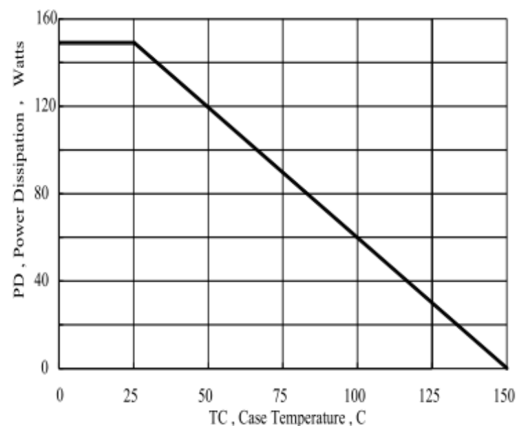
Figure 2 Maximum Power dissipation vs Case Temperature
