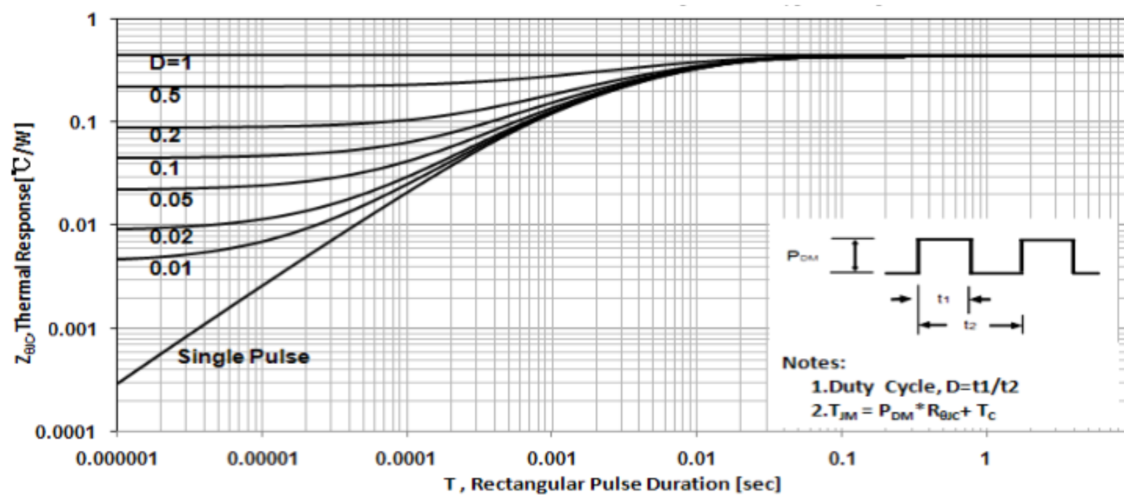
Figure 5 Maximum Effective Thermal Impedance, Junction to Case
