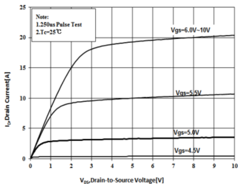
Figure 4 Typical Output Characteristics
