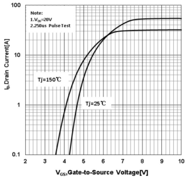
Figure 6 Typical Transfer Characteristics
