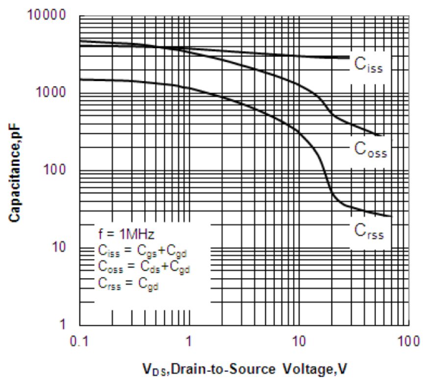
Figure 12 Typical Capacitance vs Drain to Source Voltage
