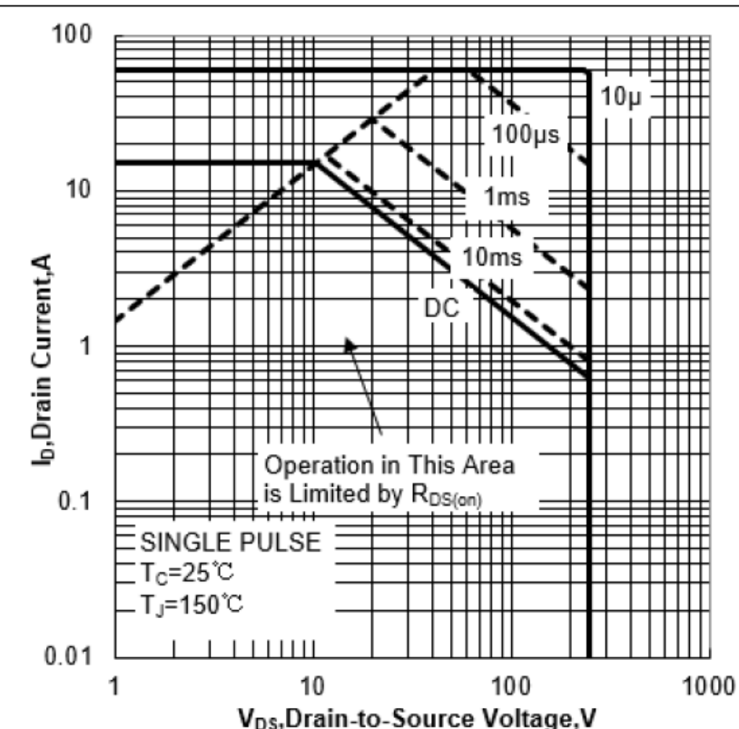
Figure 1a Safe Operating Area (No FullPAK)
