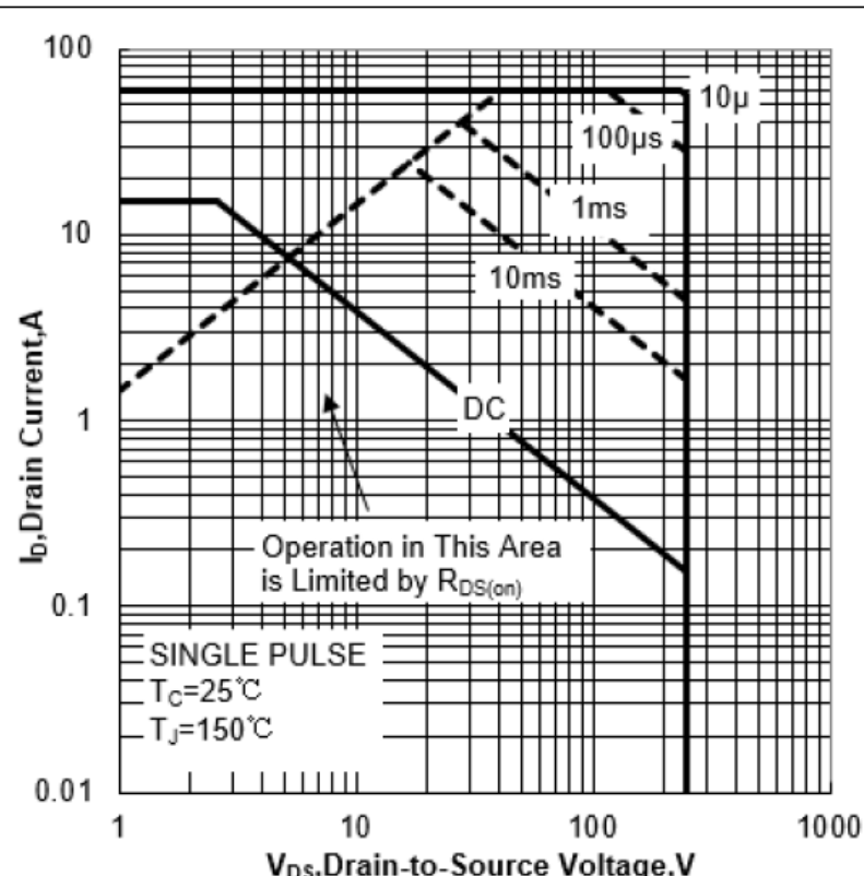
Figure 1b Safe Operating Area (FullPAK)
