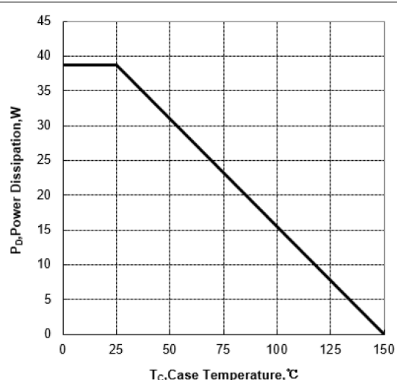
Figure 2b Power Dissipation (FullPAK)
