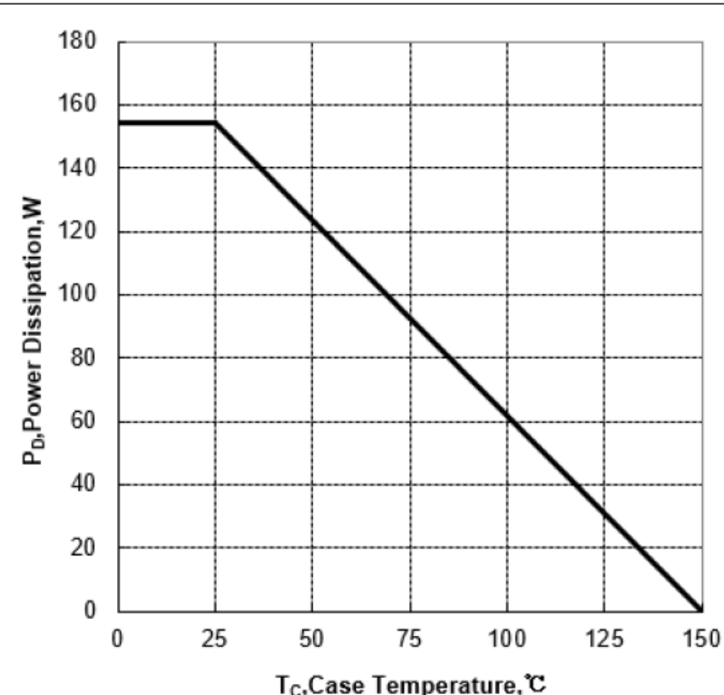
Figure 2a Power Dissipation (No FullPAK)
