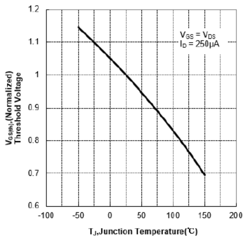
Figure 8 Typical Theshold Voltage vs Junction Temperature
