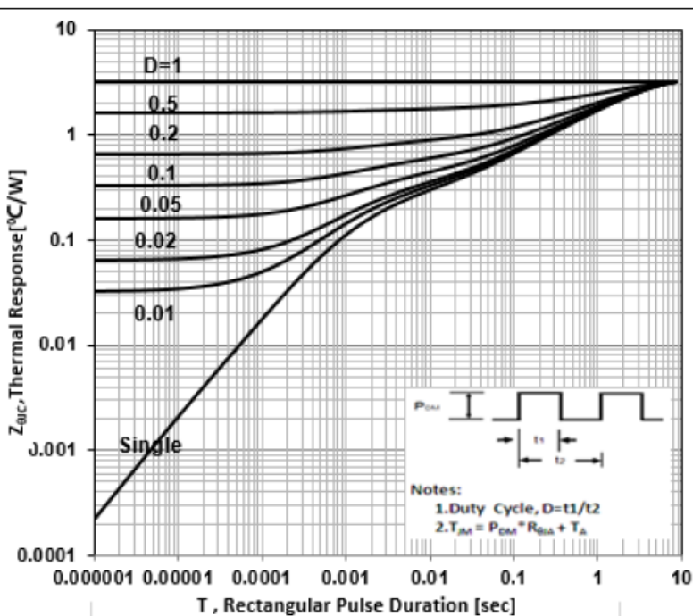
Figure 3b Max Thermal Impedance (FullPAK)
