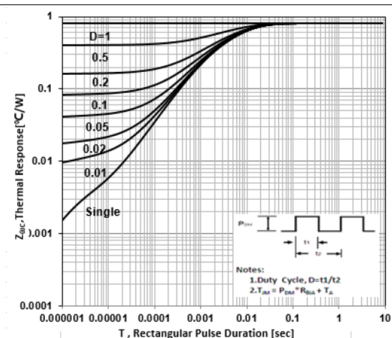
Figure 3a Max Thermal Impedance (No FullPAK)
