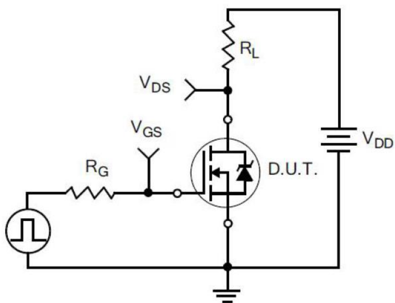
Figure 16. Resistive Switching Test Circuit
