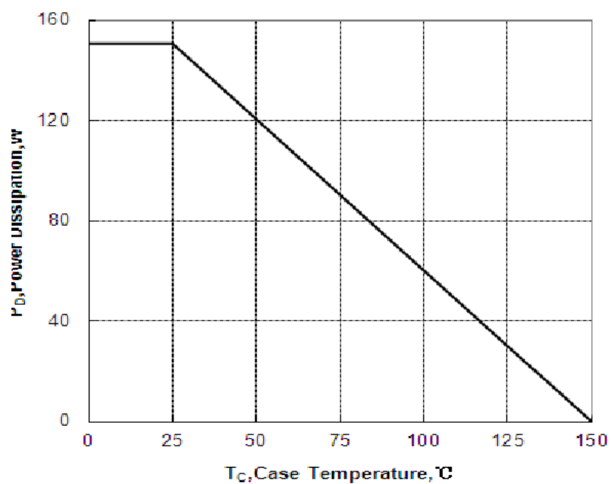
Figure 2 Maximum Power dissipation vs Case Temperature
