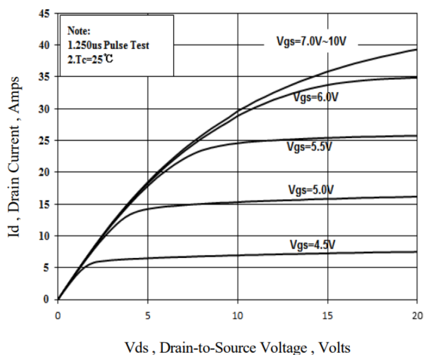
Figure 4 Typical Output Characteristics
