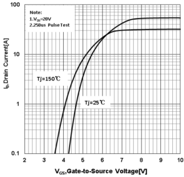
Figure 6 Typical Transfer Characteristics
