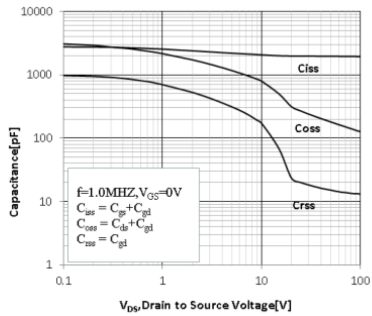
Figure 12 Typical Capacitance vs Drain to Source Voltage
