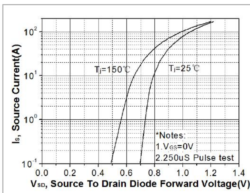
Fig. 4. On-state current vs. diode forward voltage
