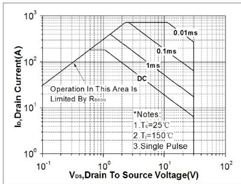
Fig. 9. Maximum safe operating area
