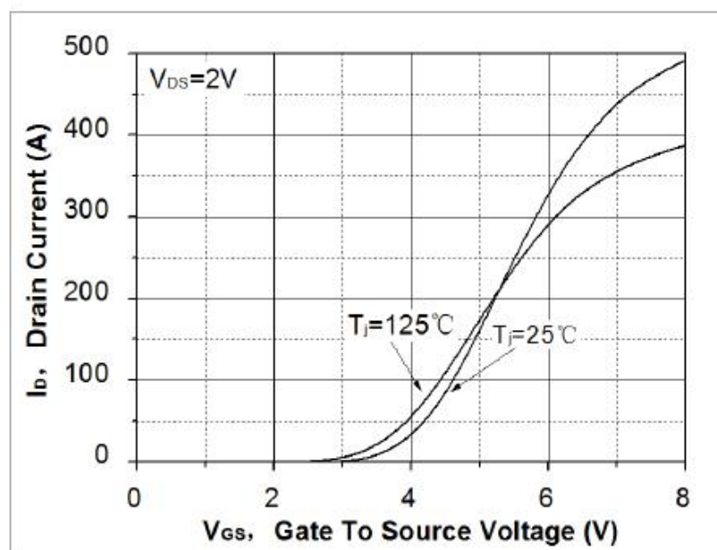
Fig. 2. Transfer Characteristics
