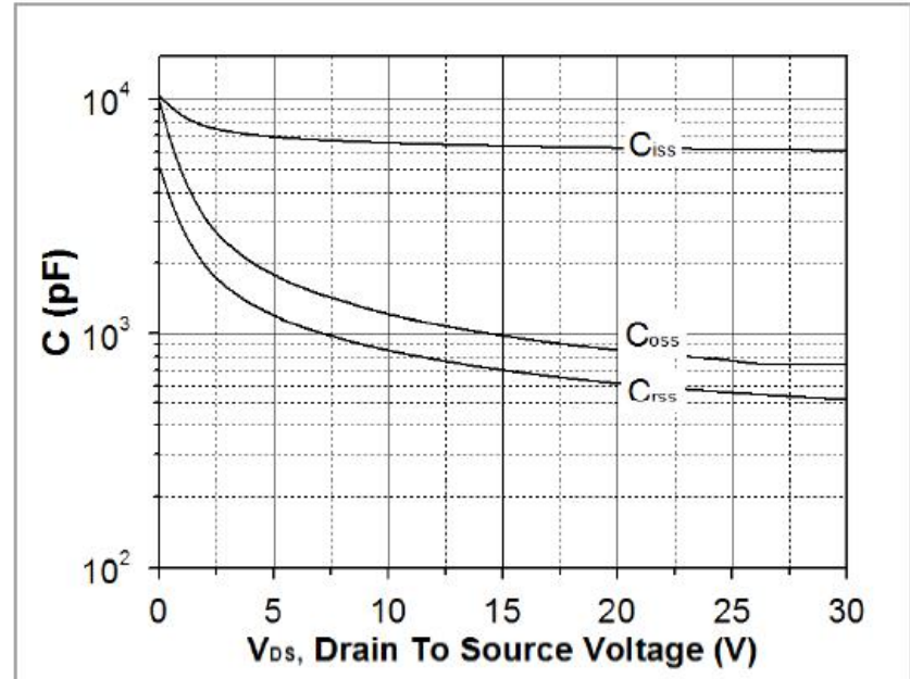
Fig. 8. Capacitance Characteristics
