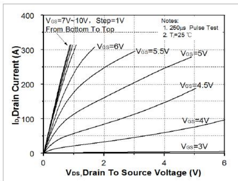
Fig. 1. On-state characteristics
