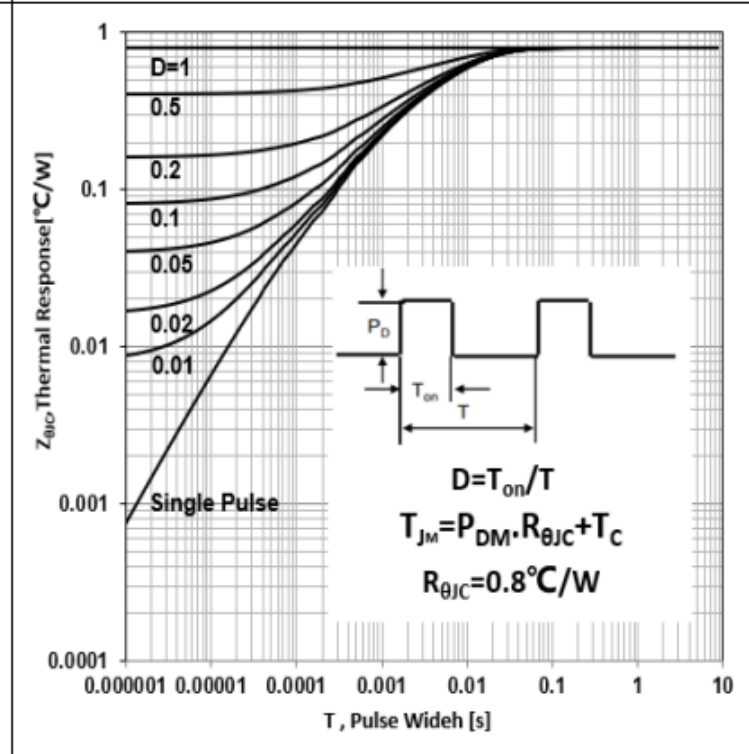
Figure 20. IGBT Transient Thermal Impedance vs Pulse Width
