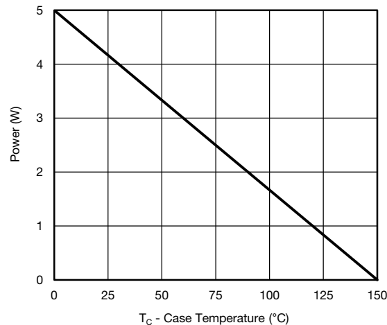
Power, Junction-to-Foot
